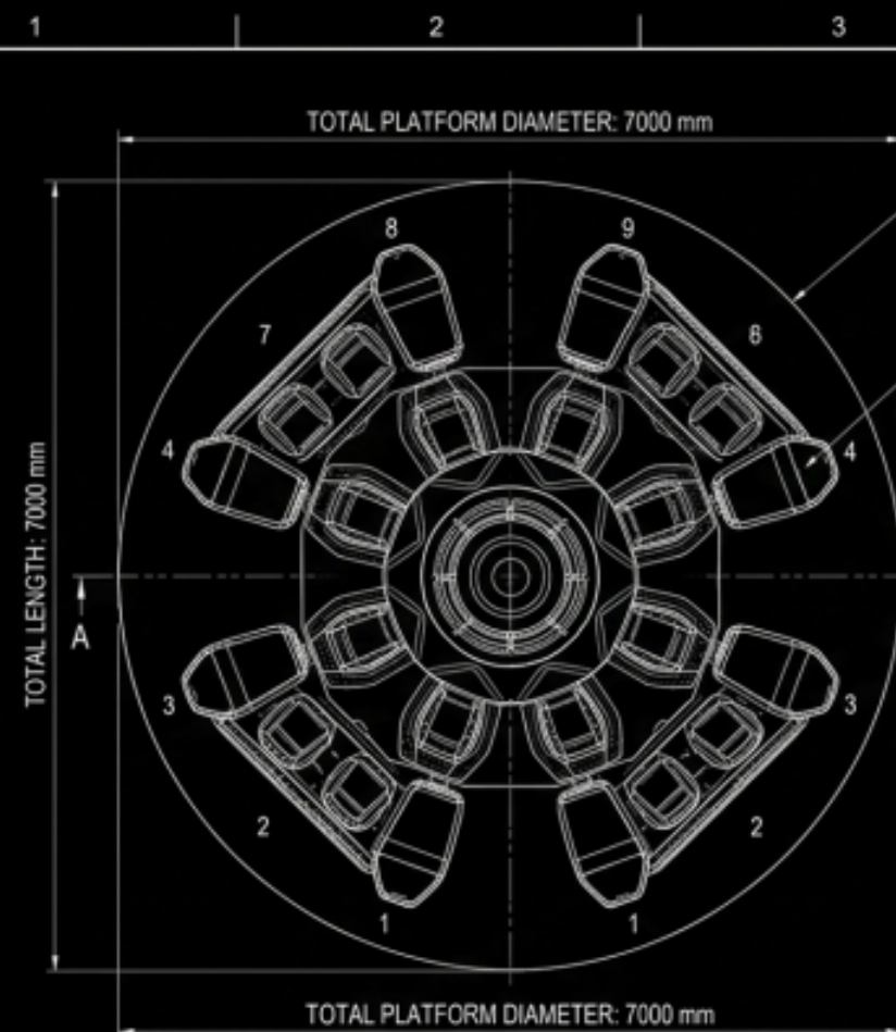
TOP VIEW
