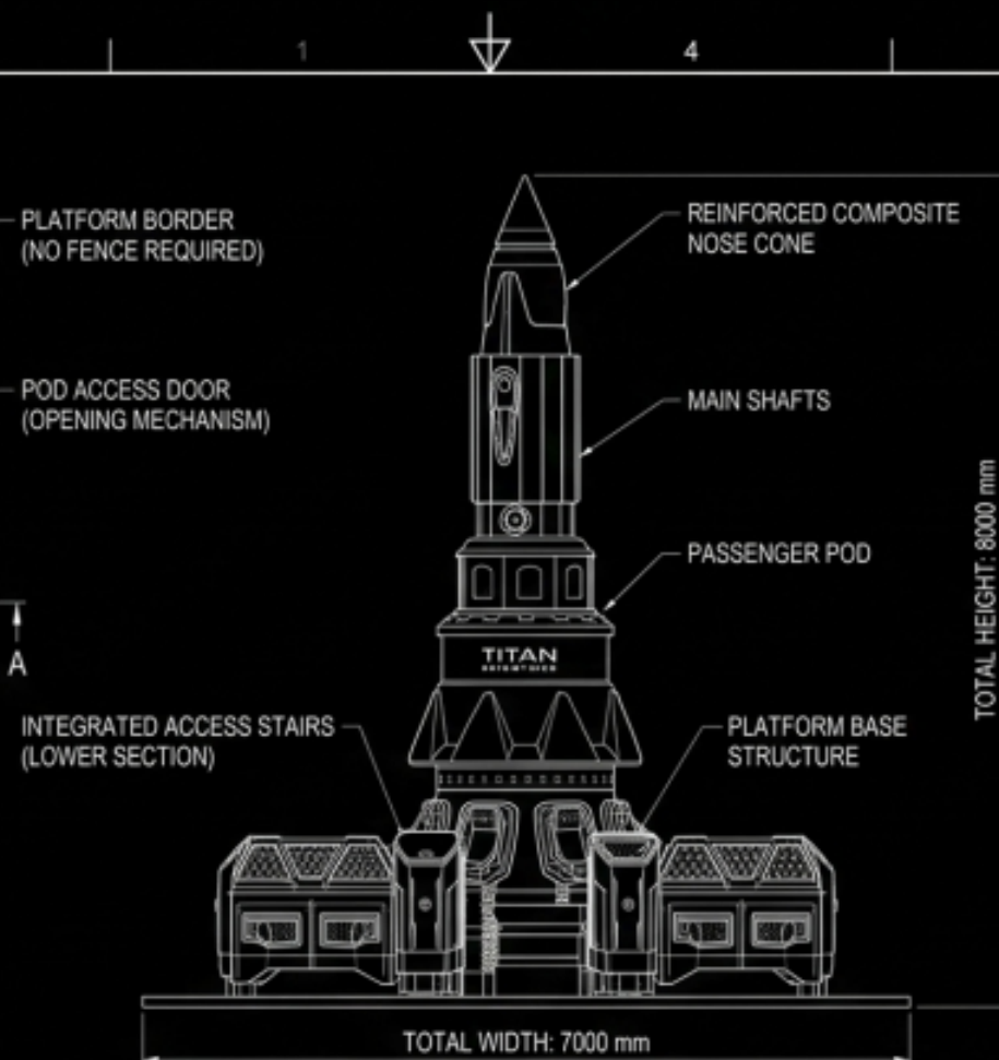
FRONT ELEVATION VIEW
