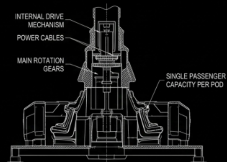
SECTIONAL VIEW (A-A)
