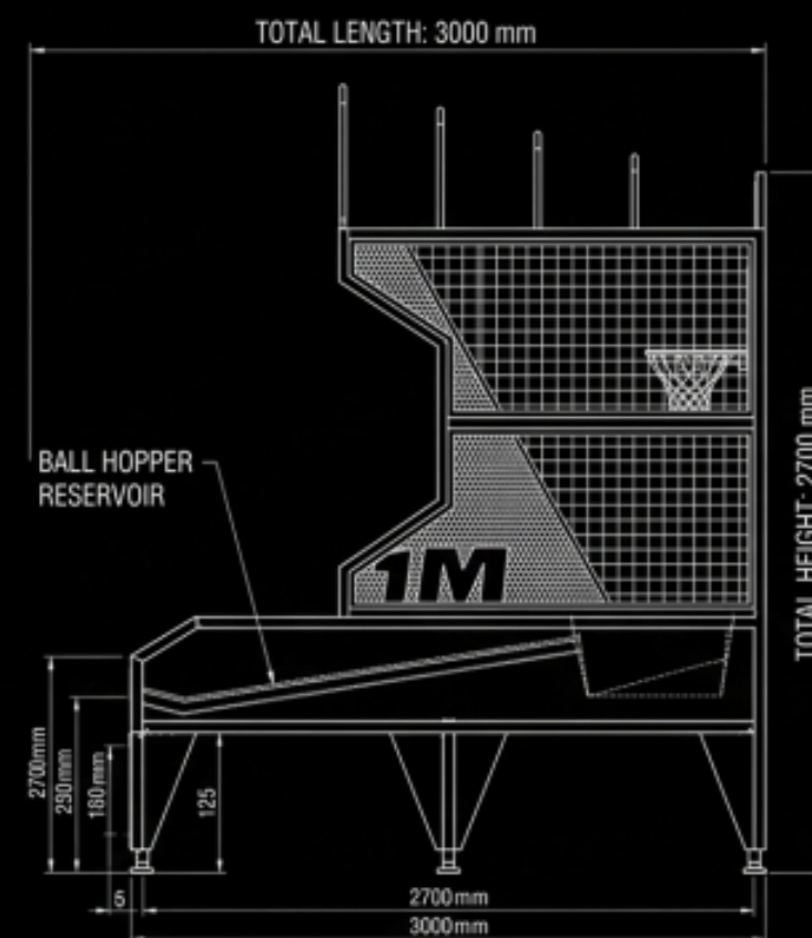
SIDE ELEVATION
