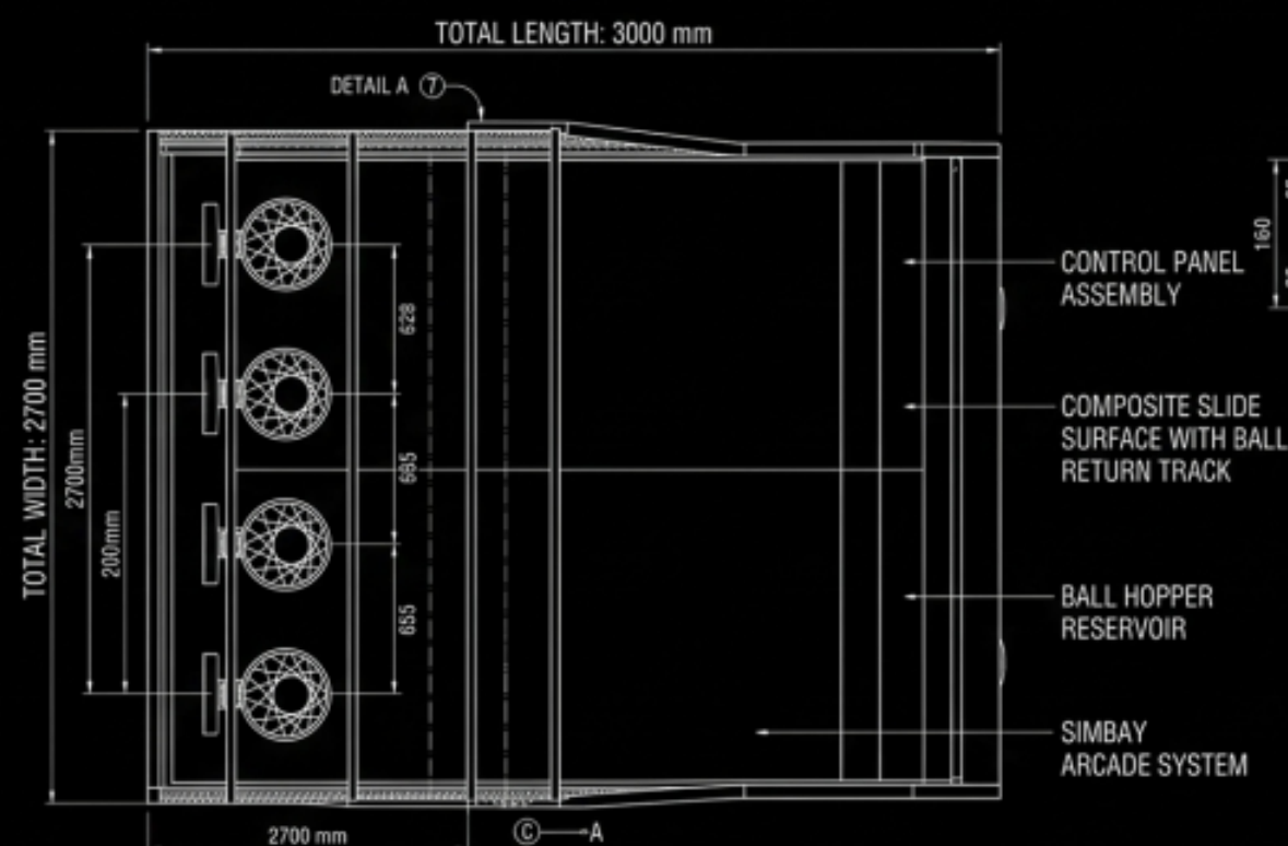
DETAILED PLAN VIEW
